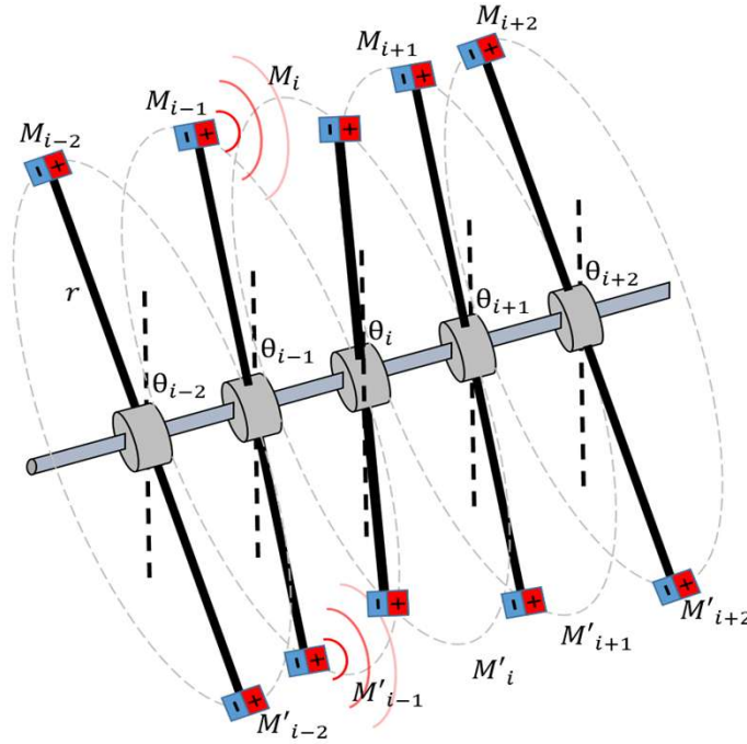
Non-linear wave equation
