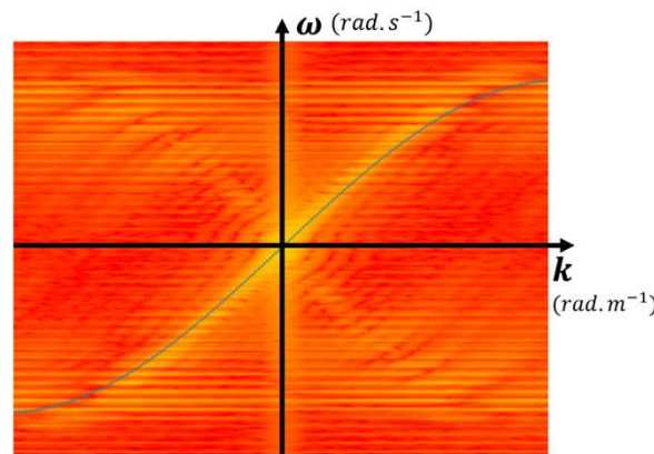
Non-linear wave equation
