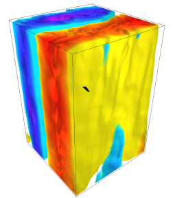
Zonal jets
