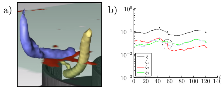
Figure 1. (a) Strong |D_l^I| (red patch) can be seen at the plane of reconnection of the blue and yellow vortex structures (b) Enstrophy \xi and its components \xi_1, \xi_2, \xi_3 versus time t .
