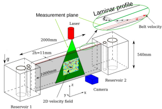
PIV setup
