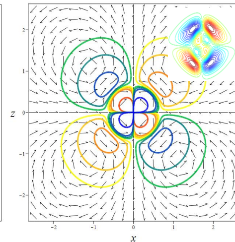
Contours for wall-normal vorticity
