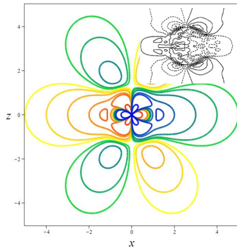
Contours for streamwise velocity
