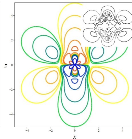
Contours for spanwise velocity
