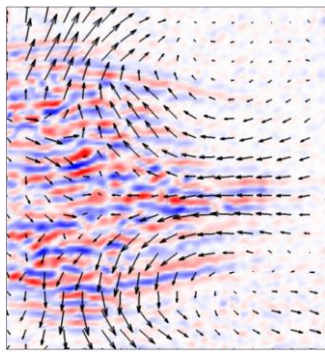
Experiment (Couliou & Monchaux 2016)
