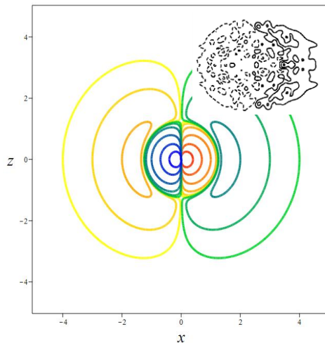
Contours for wall-normal velocity
