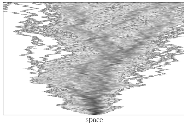
Intrinsic stochasticity of trajectories
