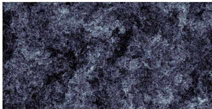
Local energy dissipation in a slice of a 3D turbulent flow at Re_\lambda = 720
