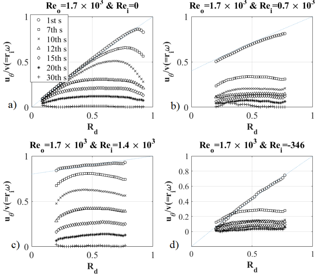
Figure 3. Decay of azimuthal velocity for different co- and counter-current configurations at different time-steps. The legend for the figures is same as that of Figure 3 (a). The dotted line represents the analytic laminar profile.
