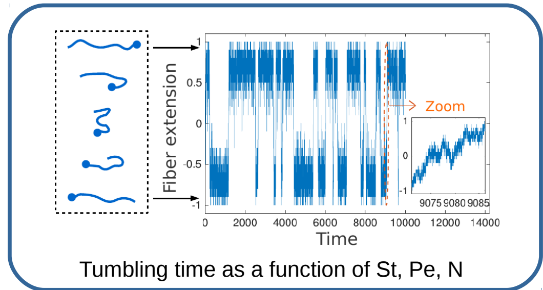
Tumbling
