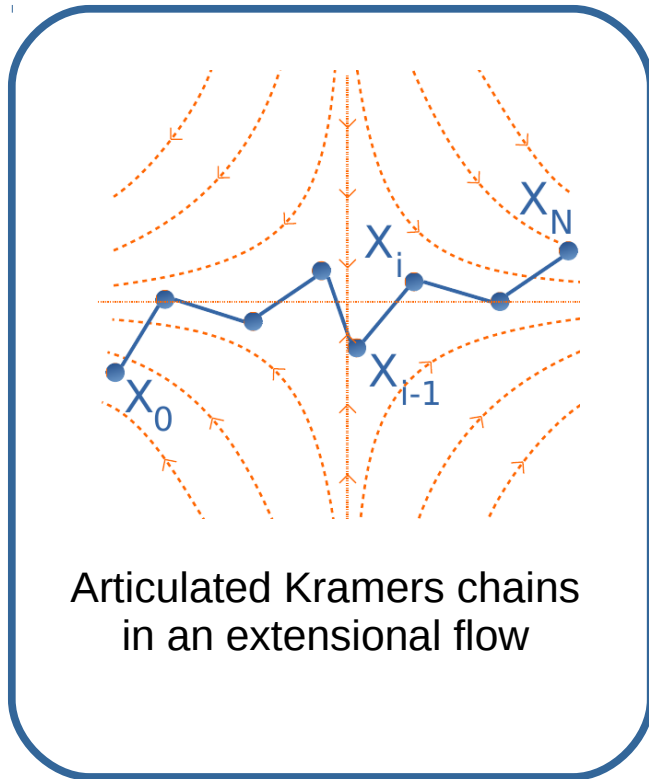
Microscopic simulations
