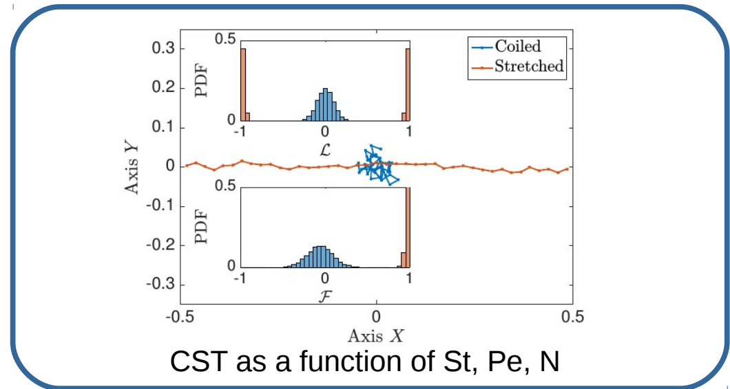
Coil-Stretch transition
