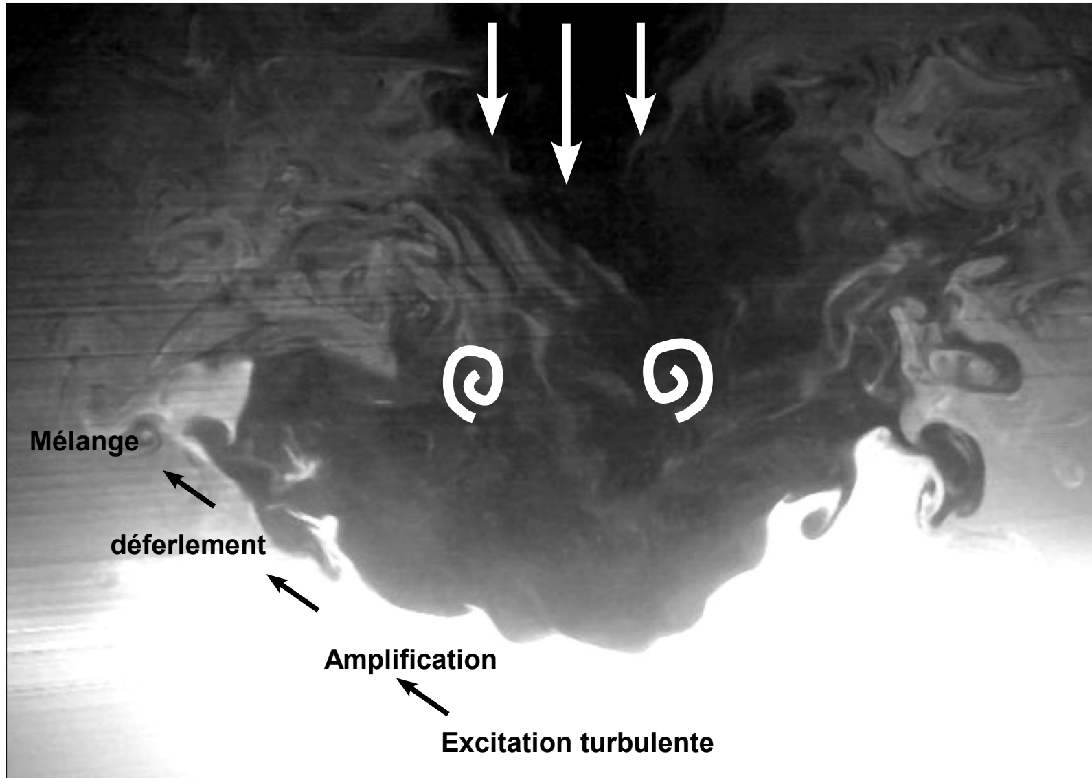
Erosion of a sharp density interface by a turbulent jet at low Froude number, Herault et al, soumis à J.F.M.
