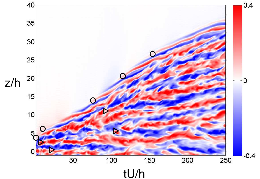
Numerical space-time diagram: U_x
